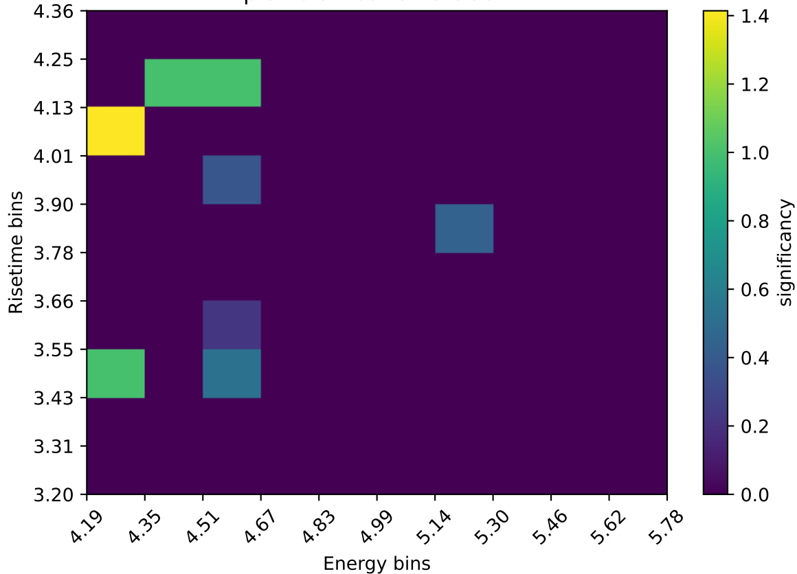
pion distribution 5.0GeV
